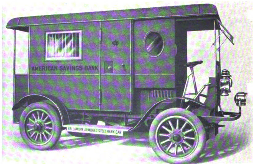
Armored Steel Motor Bank Car Type 11 VC. Side View
